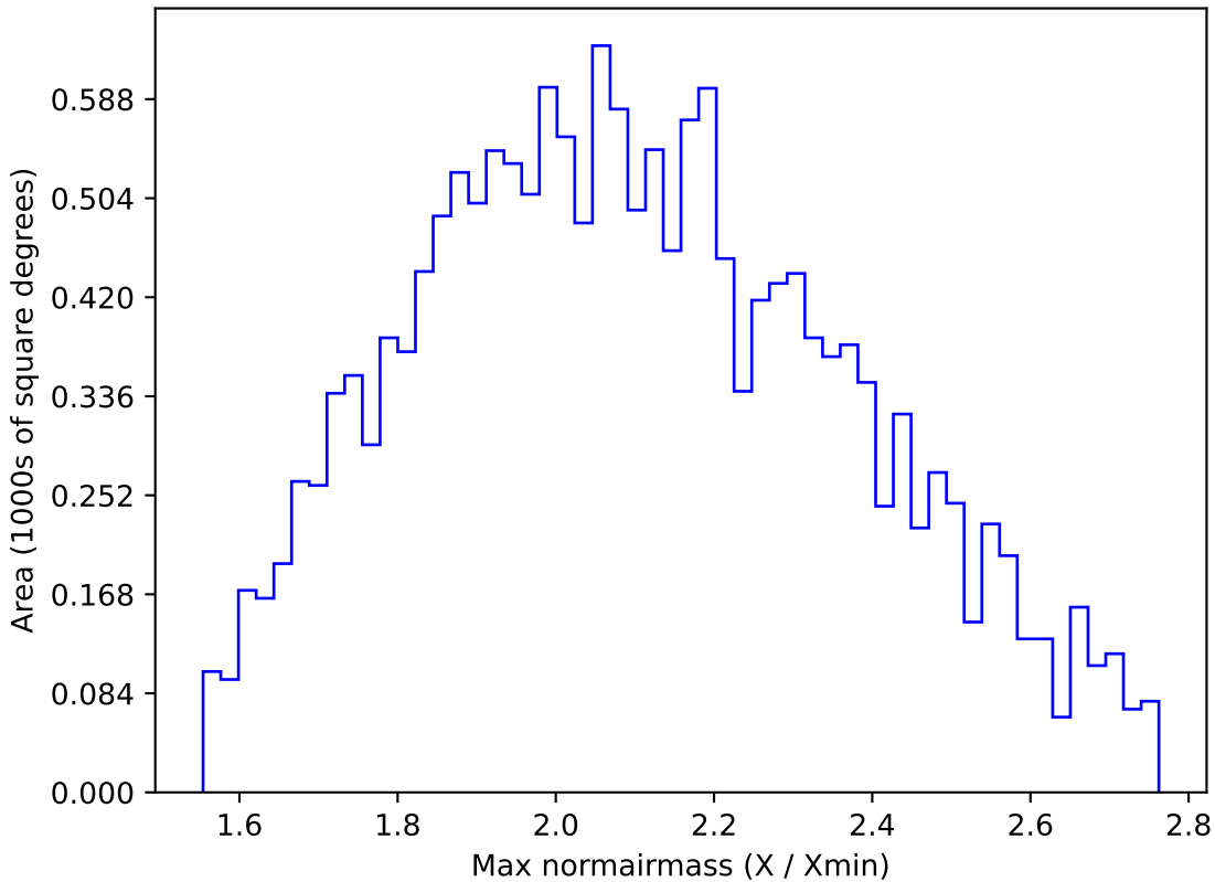
too_elab_r64_d2_giz_v3.4_10yrs WFD y band: Max normairmass
