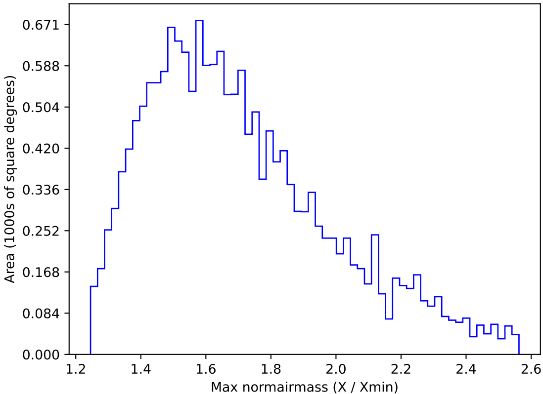
too_elab_r64_d2_giz_v3.4_10yrs WFD u band: Max normairmass
