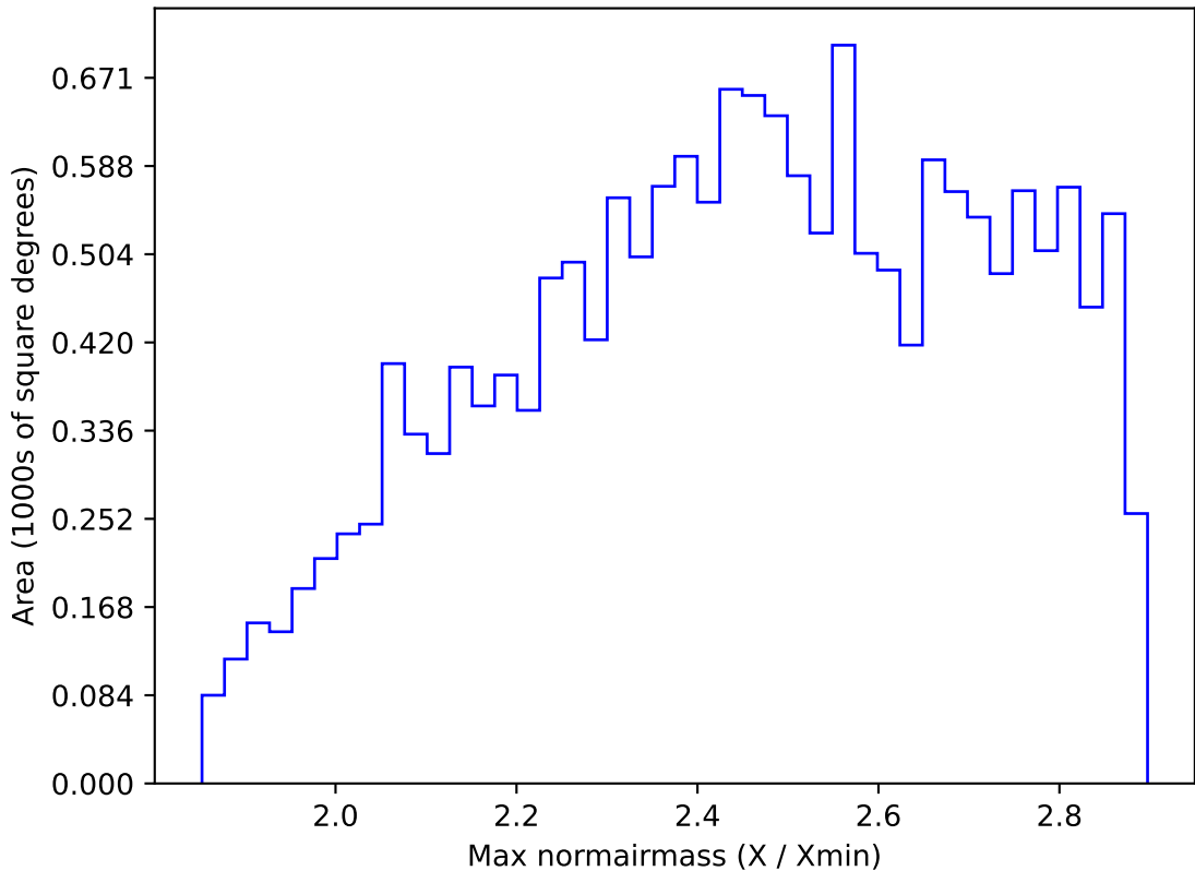
too_elab_r64_d2_giz_v3.4_10yrs WFD all bands: Max normairmass
