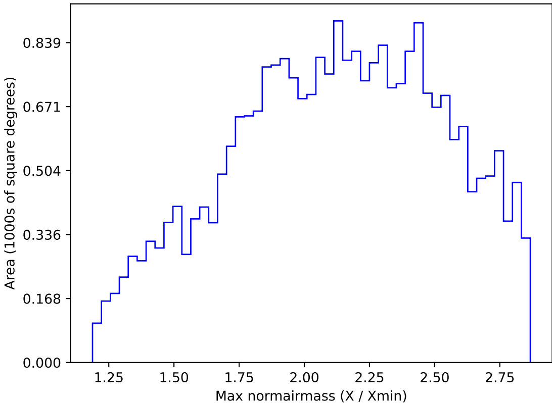
too_elab_r64_d2_giz_v3.4_10yrs All sky z band: Max normairmass
