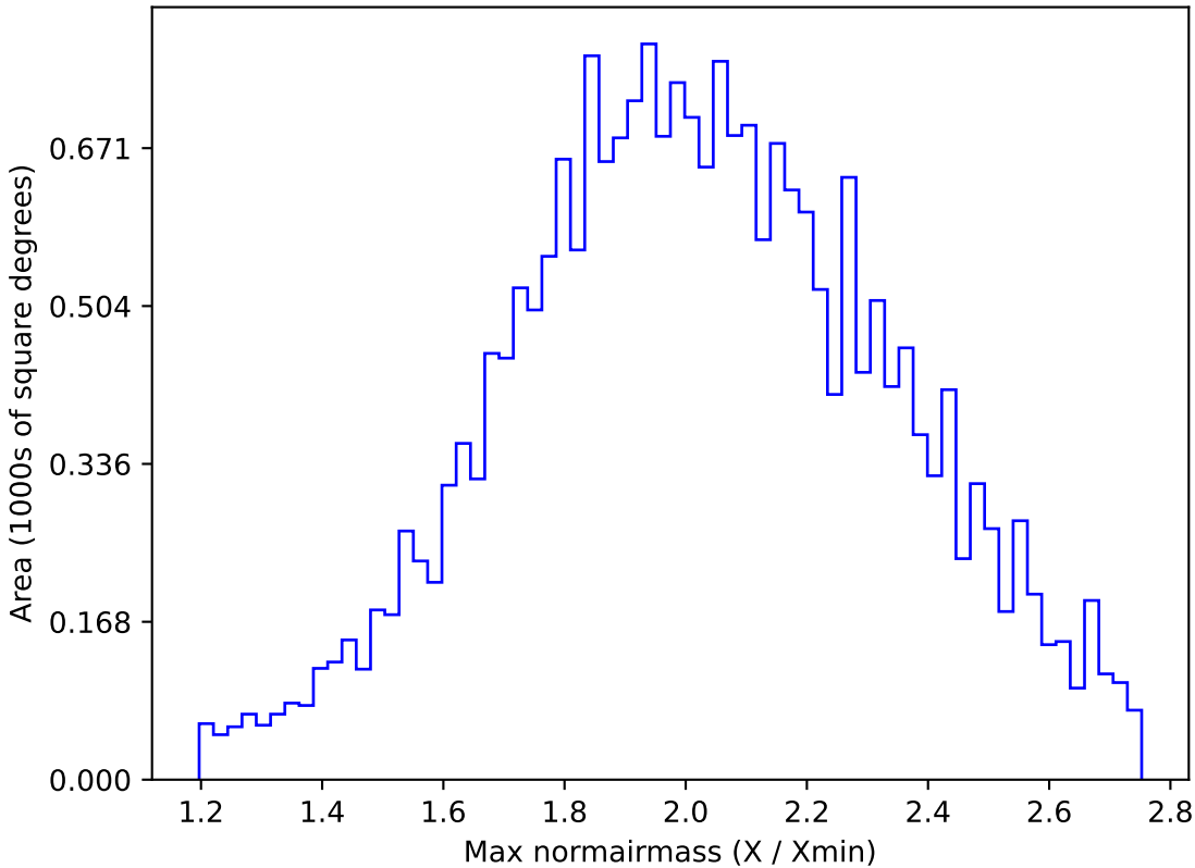
too_elab_r64_d2_giz_v3.4_10yrs All sky y band: Max normairmass
