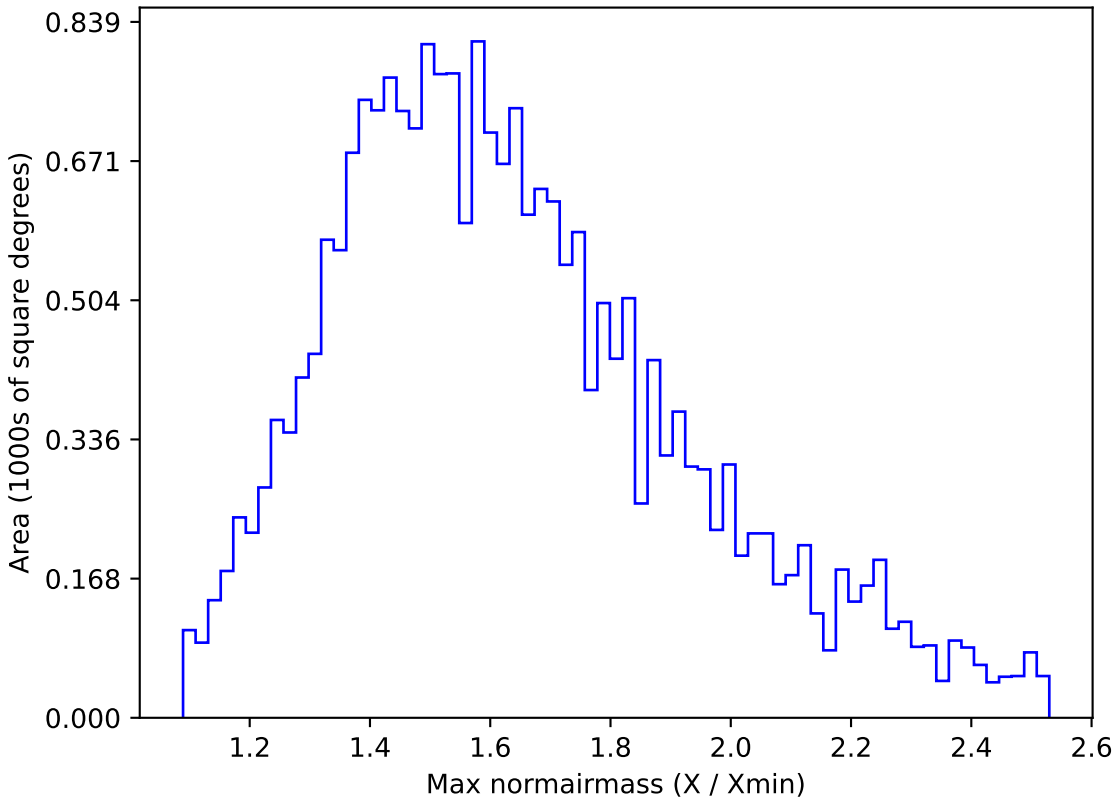
too_elab_r64_d2_giz_v3.4_10yrs All sky u band: Max normairmass
