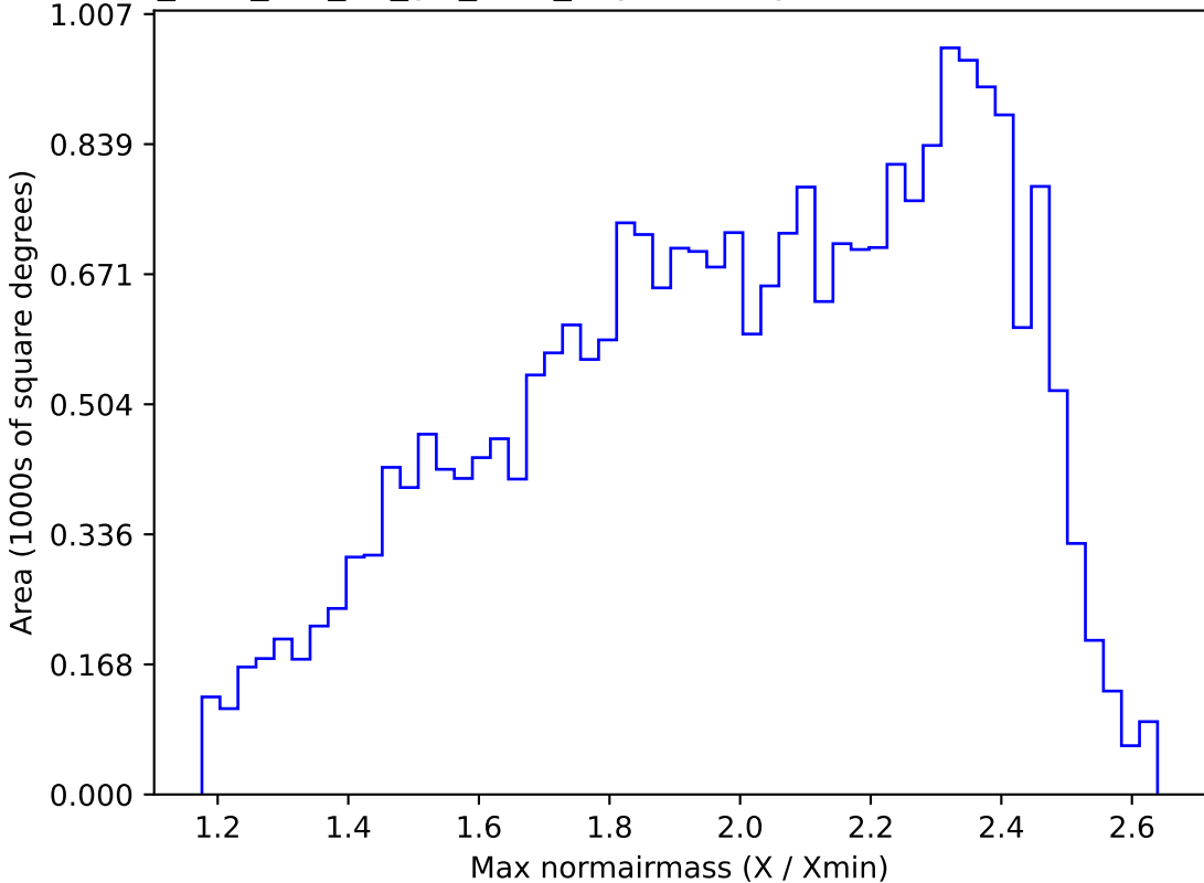
too_elab_r64_d2_giz_v3.4_10yrs All sky r band: Max normairmass
