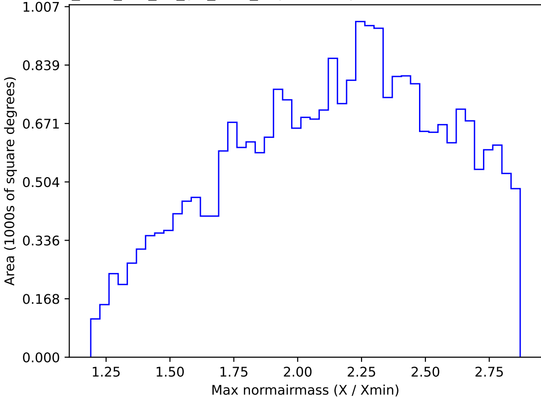
too_elab_r64_d2_giz_v3.4_10yrs All sky i band: Max normairmass
