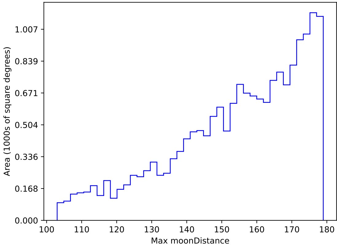
too_elab_r64_d2_giz_v3.4_10yrs WFD z band: Max moonDistance
