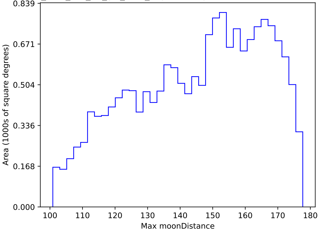
too_elab_r64_d2_giz_v3.4_10yrs WFD y band: Max moonDistance
