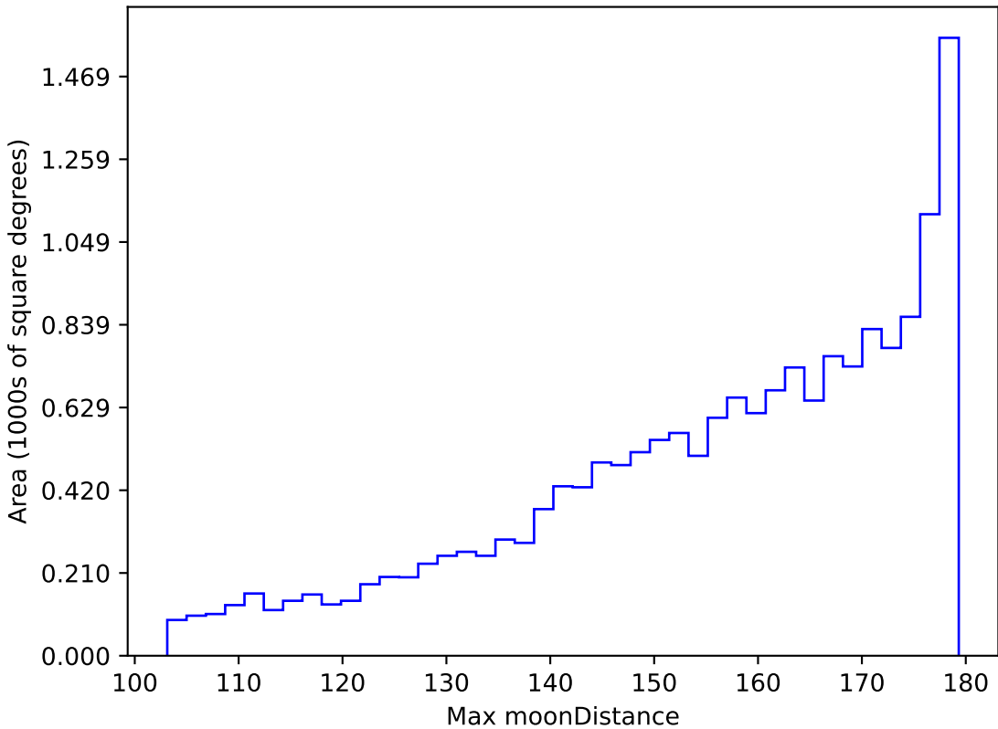
too_elab_r64_d2_giz_v3.4_10yrs WFD r band: Max moonDistance
