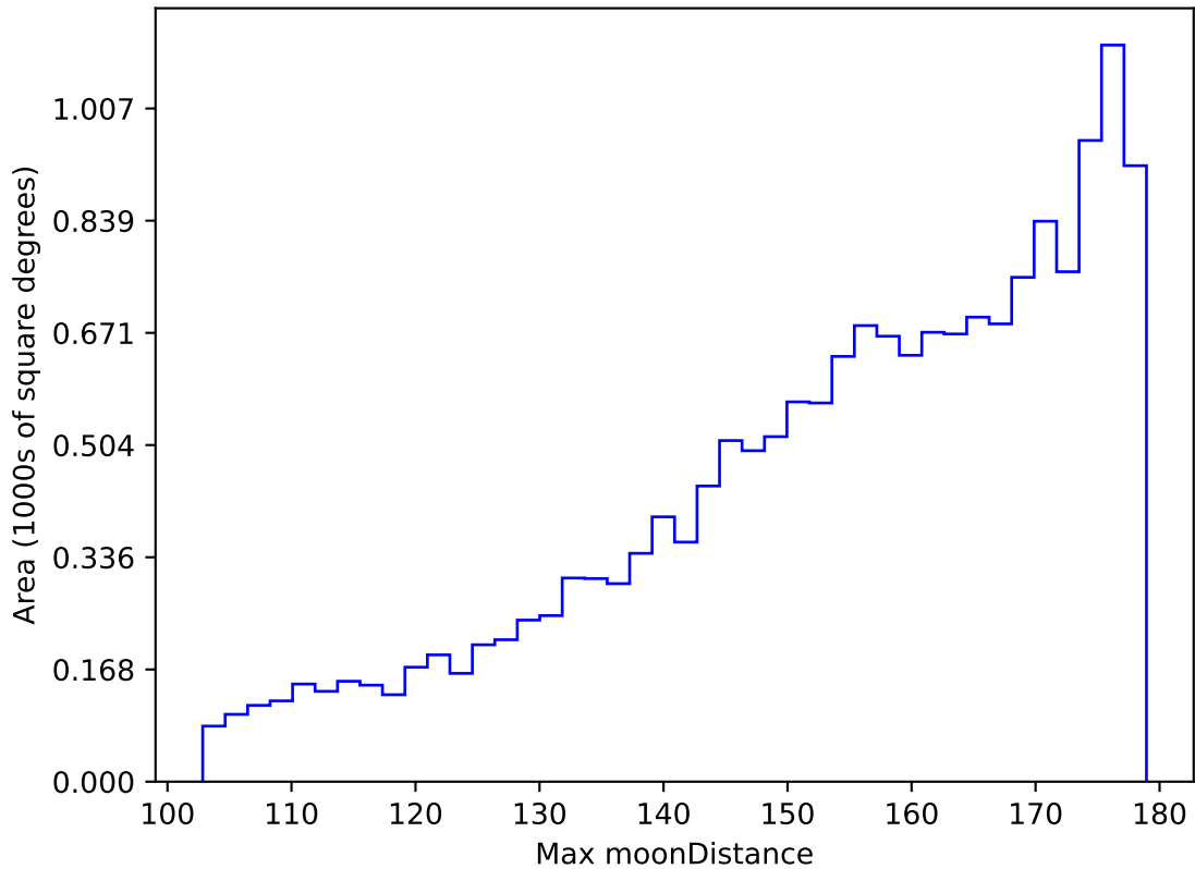
too_elab_r64_d2_giz_v3.4_10yrs WFD g band: Max moonDistance
