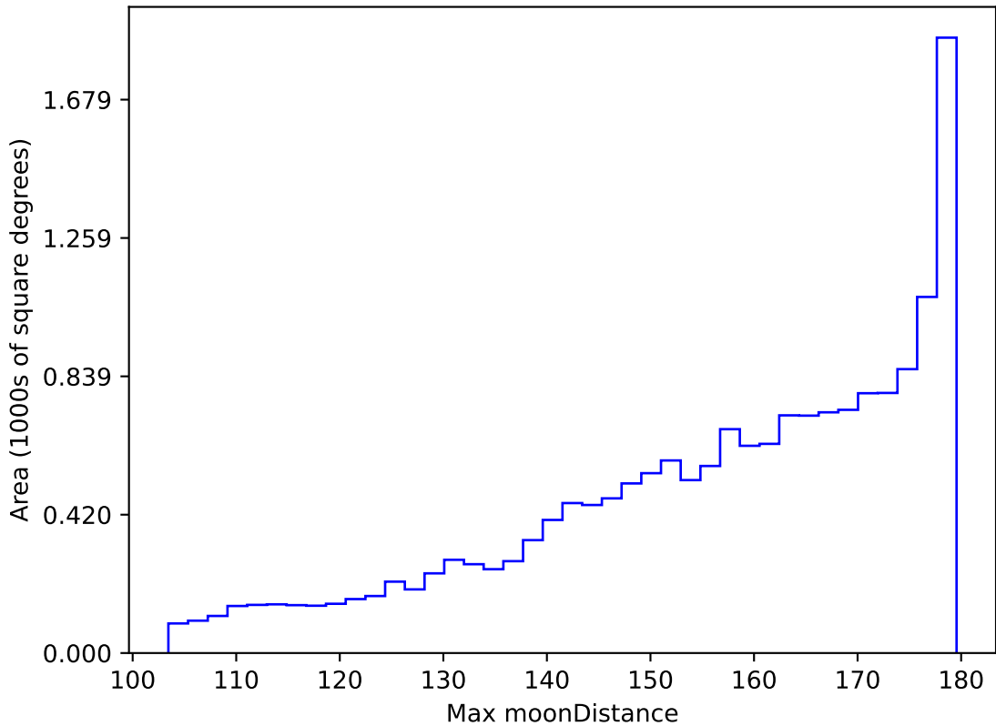
too_elab_r64_d2_giz_v3.4_10yrs WFD all bands: Max moonDistance
