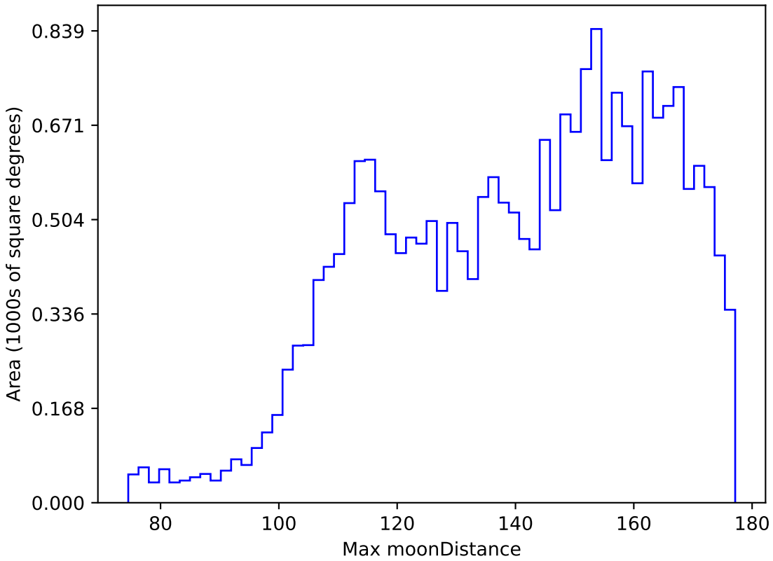
too_elab_r64_d2_giz_v3.4_10yrs All sky y band: Max moonDistance
