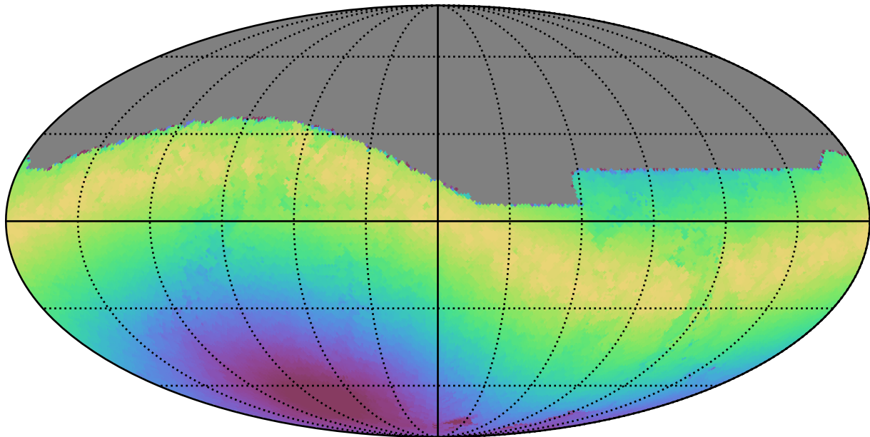
too_elab_r64_d2_giz_v3.4_10yrs All sky i band: Max moonDistance
