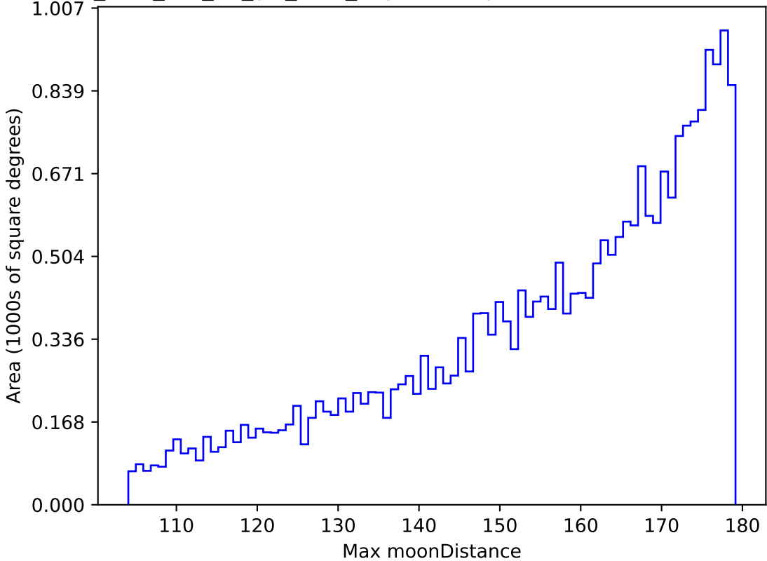
too_elab_r64_d2_giz_v3.4_10yrs All sky i band: Max moonDistance
