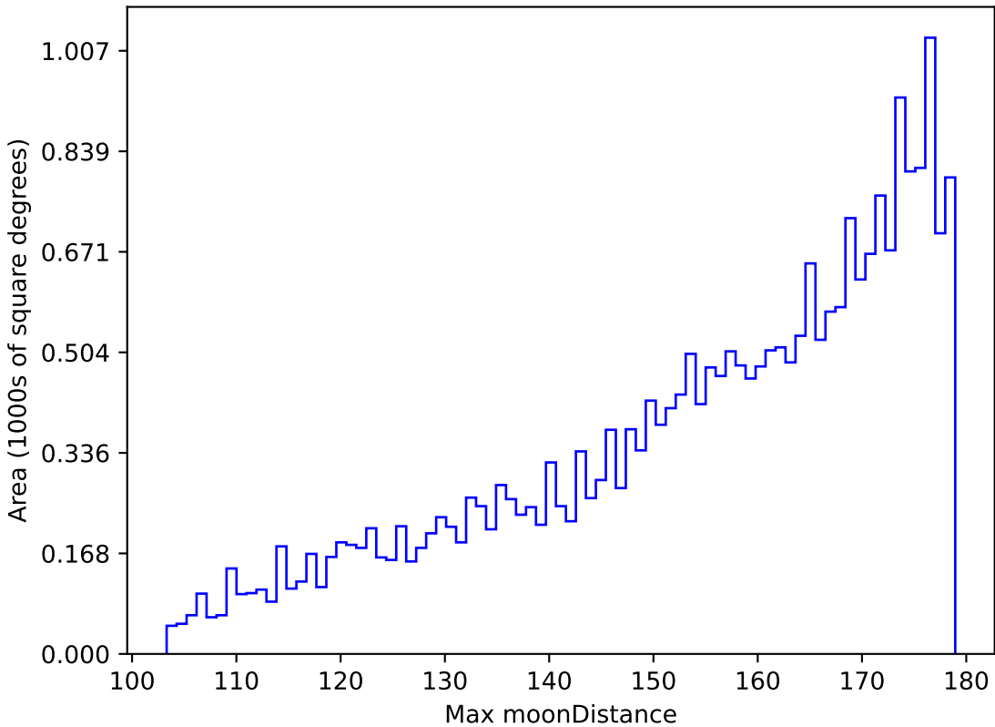
too_elab_r64_d2_giz_v3.4_10yrs All sky g band: Max moonDistance
