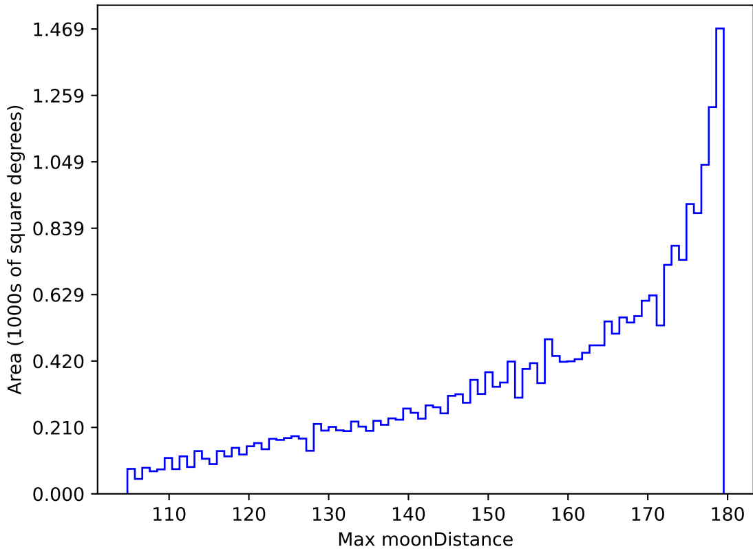
too_elab_r64_d2_giz_v3.4_10yrs All sky all bands: Max moonDistance
