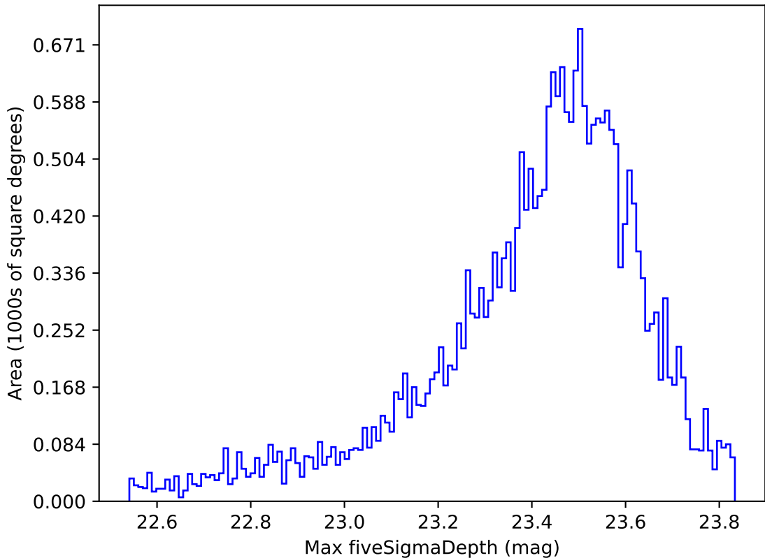
too_elab_r64_d2_giz_v3.4_10yrs Yr 1 z band: Max fiveSigmaDepth
