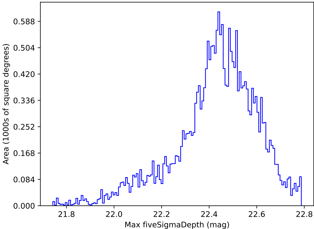
too_elab_r64_d2_giz_v3.4_10yrs Yr 1 y band: Max fiveSigmaDepth
