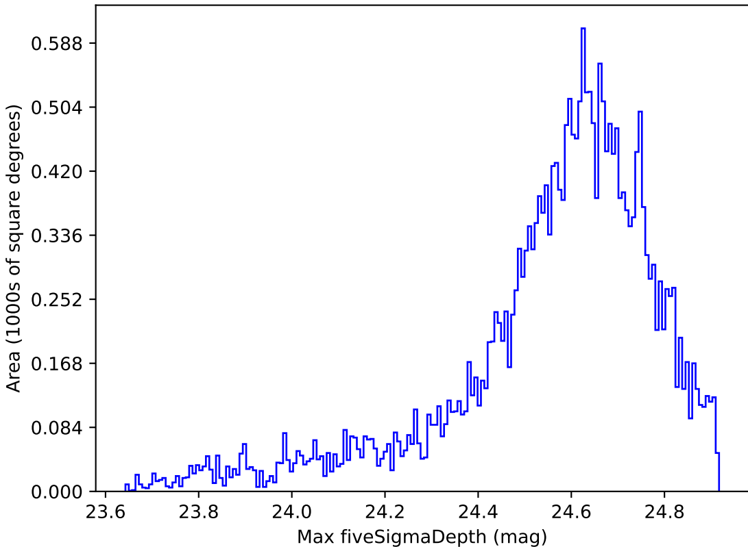
too_elab_r64_d2_giz_v3.4_10yrs Yr 1 r band: Max fiveSigmaDepth
