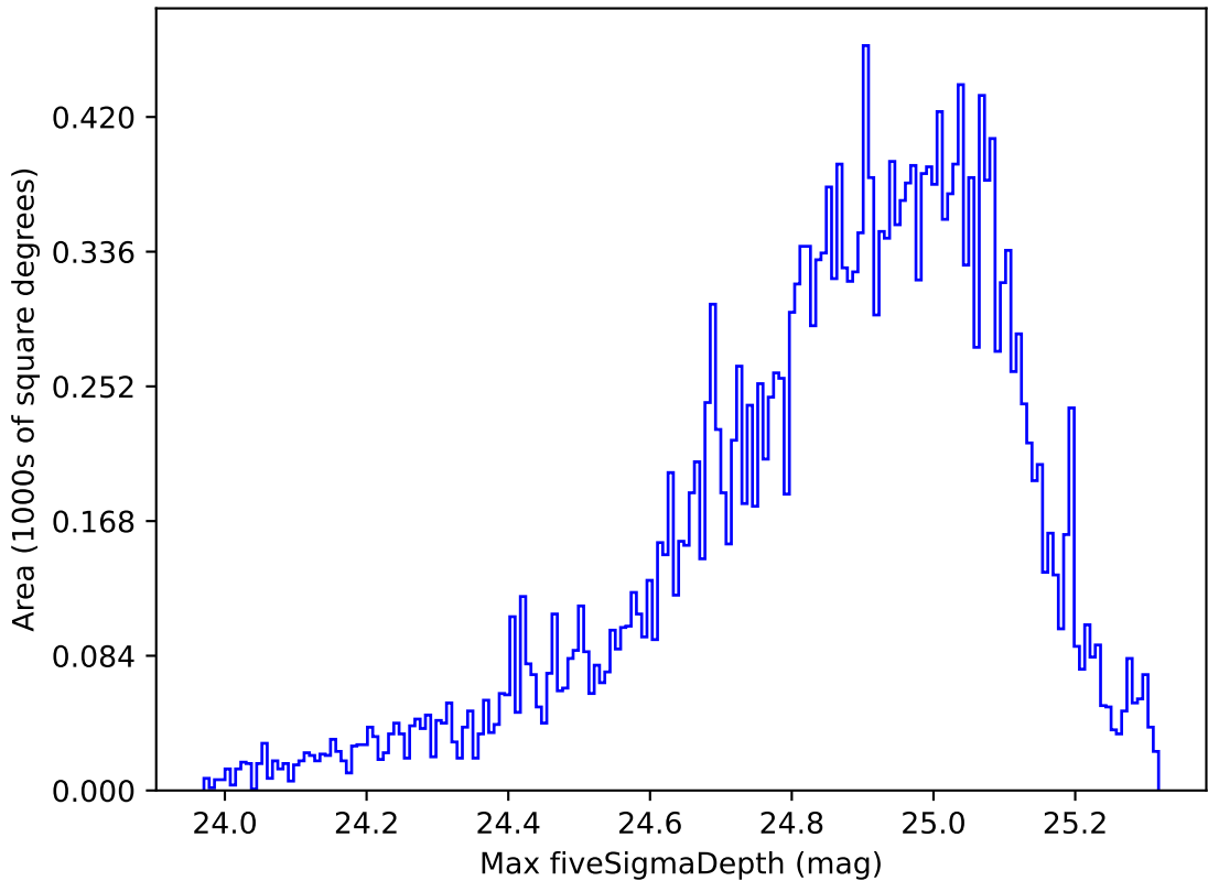
too_elab_r64_d2_giz_v3.4_10yrs Yr 1 g band: Max fiveSigmaDepth
