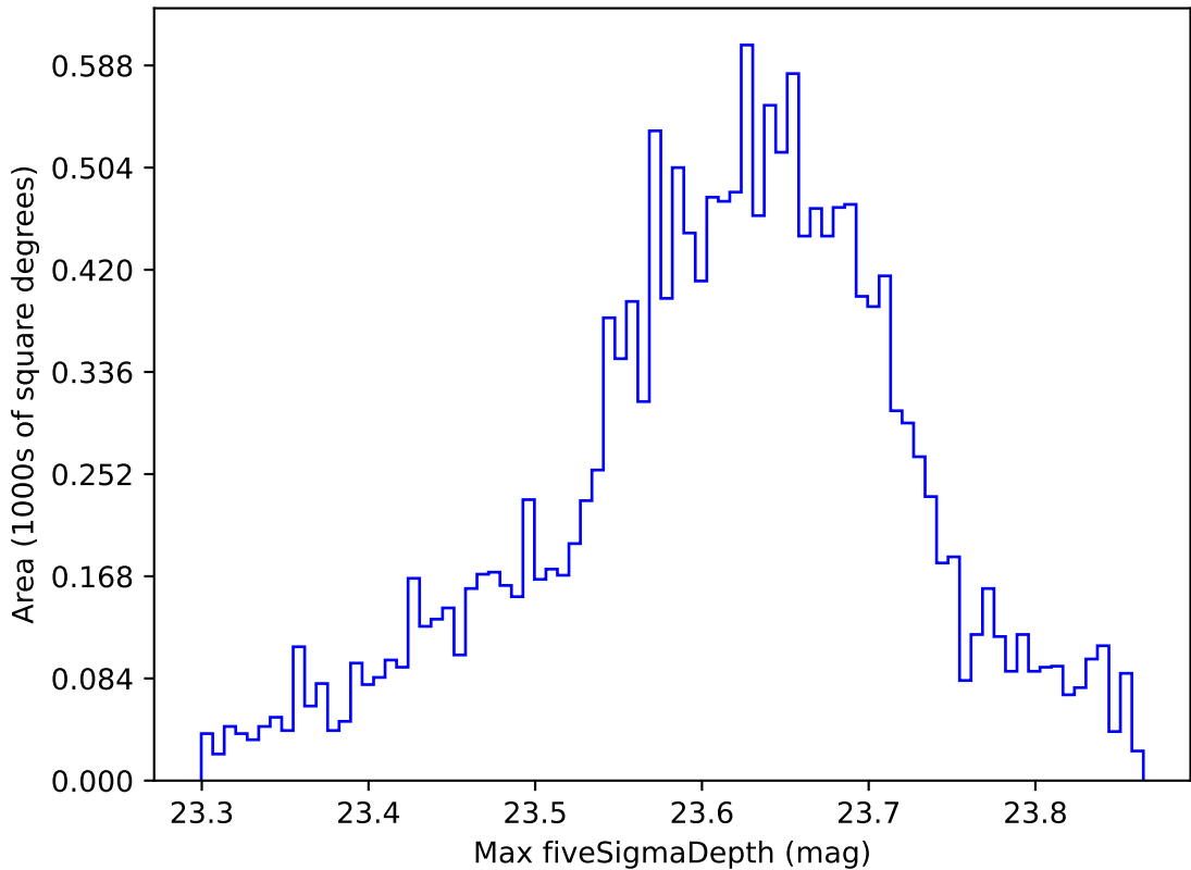
too_elab_r64_d2_giz_v3.4_10yrs WFD z band: Max fiveSigmaDepth
