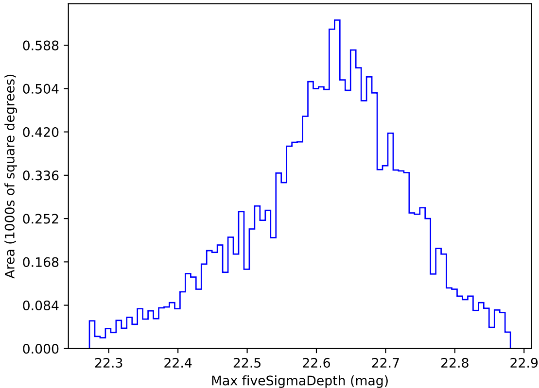
too_elab_r64_d2_giz_v3.4_10yrs WFD y band: Max fiveSigmaDepth
