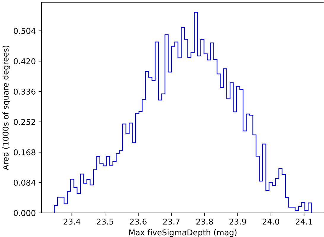
too_elab_r64_d2_giz_v3.4_10yrs WFD u band: Max fiveSigmaDepth
