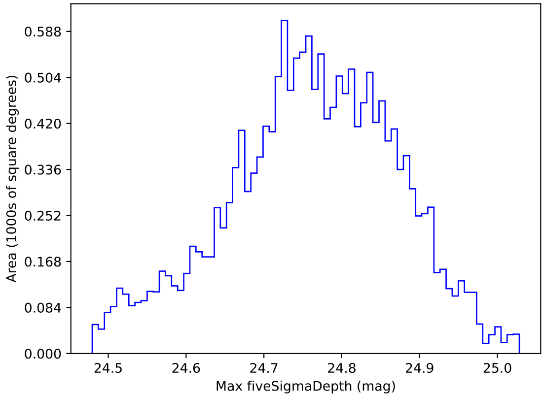
too_elab_r64_d2_giz_v3.4_10yrs WFD r band: Max fiveSigmaDepth
