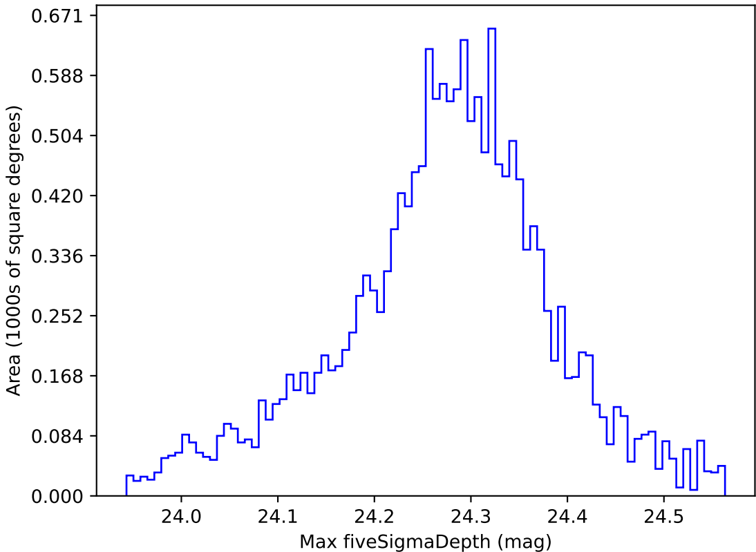
too_elab_r64_d2_giz_v3.4_10yrs WFD i band: Max fiveSigmaDepth
