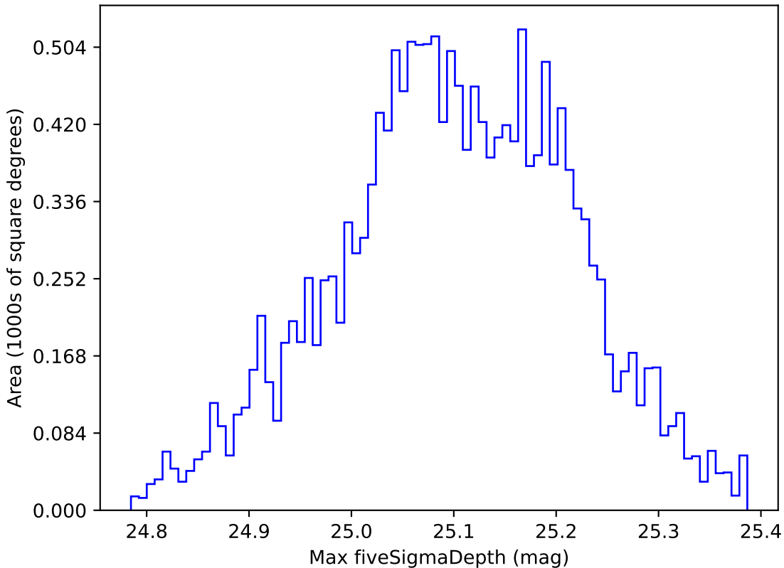
too_elab_r64_d2_giz_v3.4_10yrs WFD g band: Max fiveSigmaDepth
