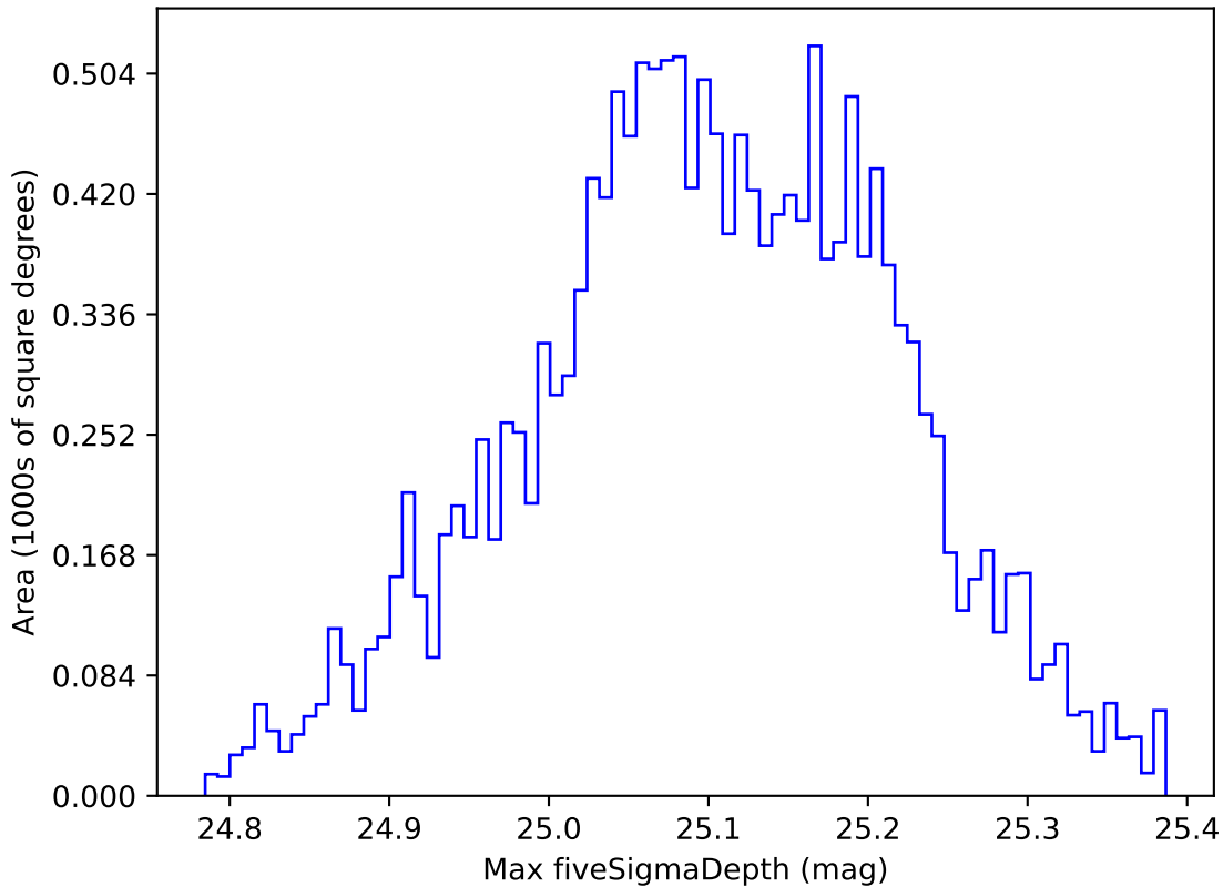
too_elab_r64_d2_giz_v3.4_10yrs WFD all bands: Max fiveSigmaDepth
