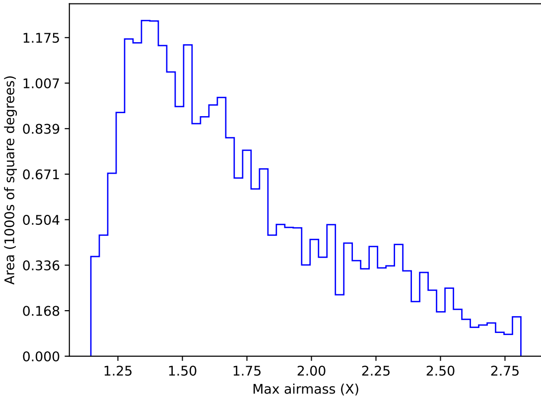
too_elab_r64_d2_giz_v3.4_10yrs Yr 1 z band: Max airmass
