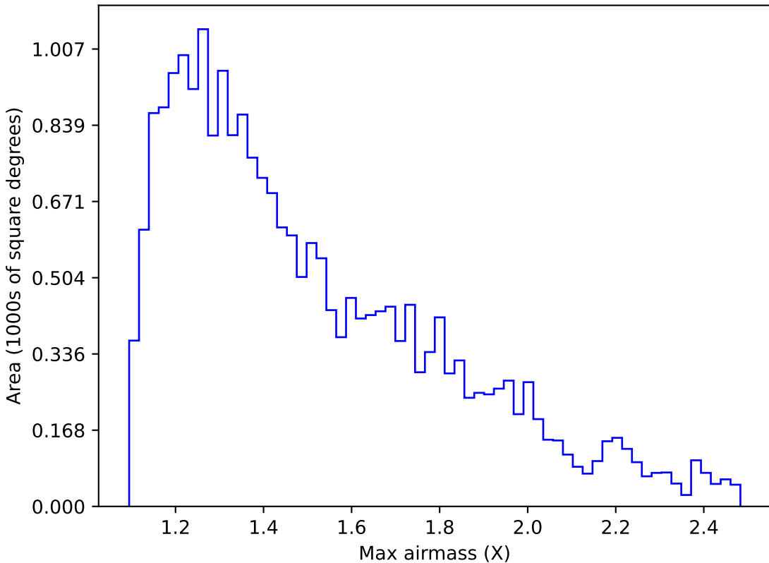
too_elab_r64_d2_giz_v3.4_10yrs Yr 1 u band: Max airmass
