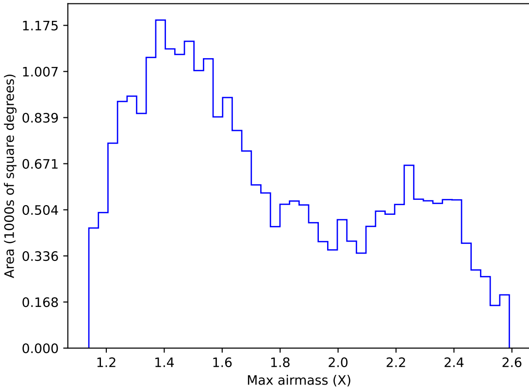
too_elab_r64_d2_giz_v3.4_10yrs Yr 1 r band: Max airmass
