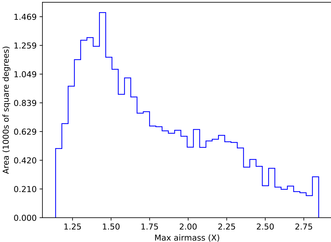
too_elab_r64_d2_giz_v3.4_10yrs Yr 1 i band: Max airmass
