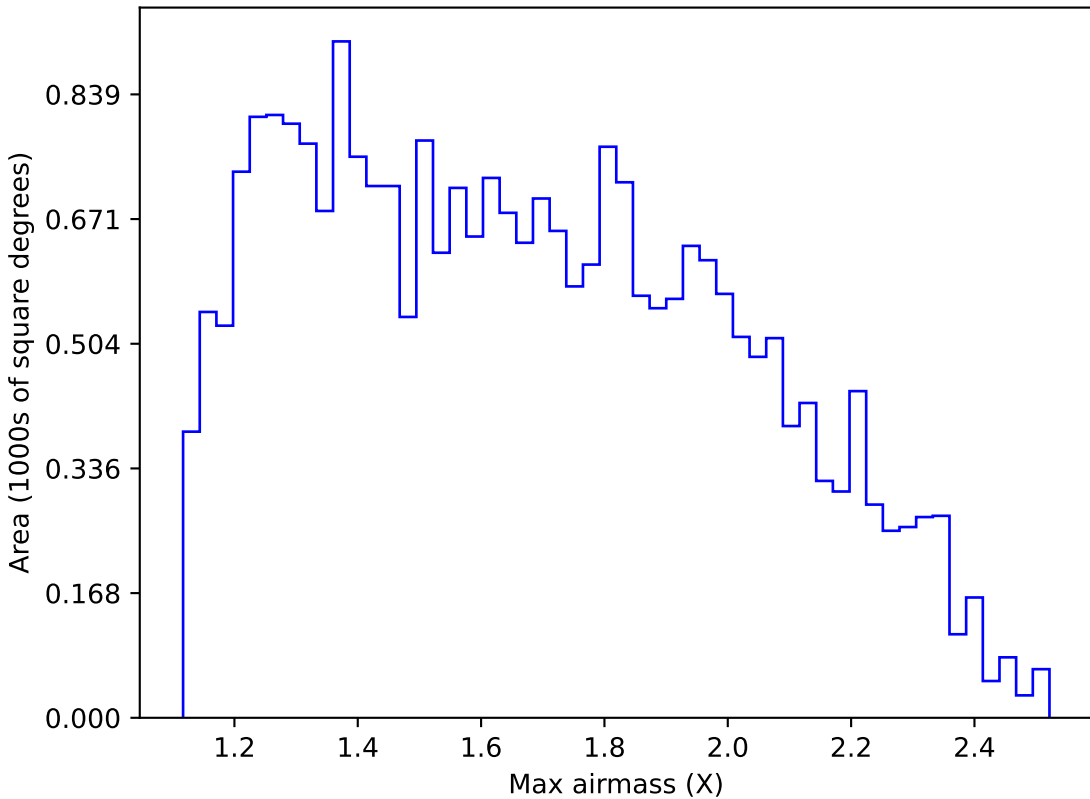
too_elab_r64_d2_giz_v3.4_10yrs Yr 1 g band: Max airmass
