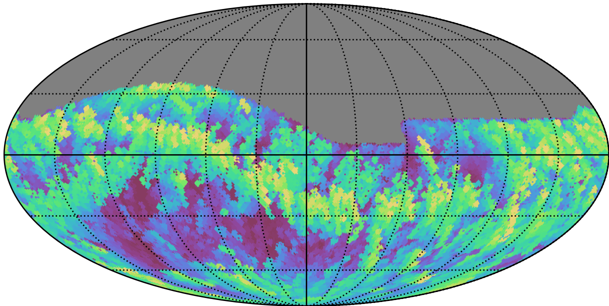
too_elab_r64_d2_giz_v3.4_10yrs Yr 1 all bands: Max airmass
