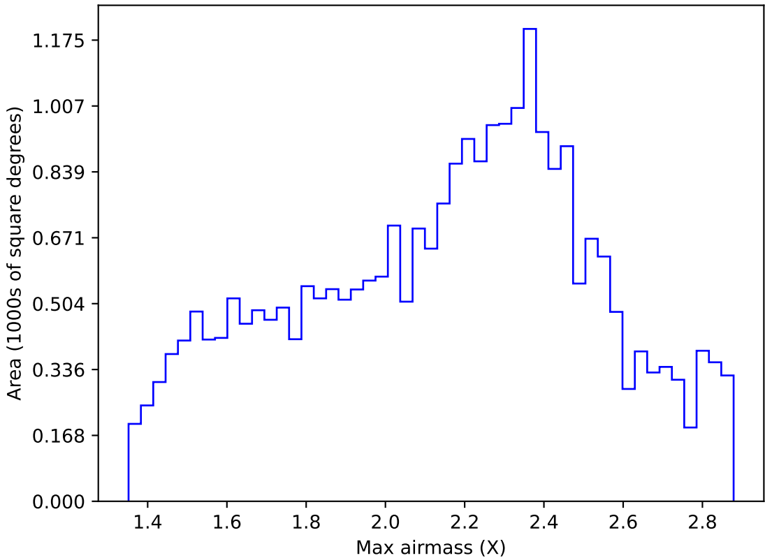
too_elab_r64_d2_giz_v3.4_10yrs Yr 1 all bands: Max airmass
