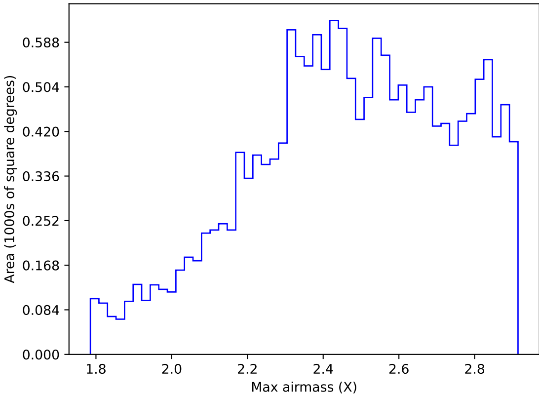
too_elab_r64_d2_giz_v3.4_10yrs WFD z band: Max airmass
