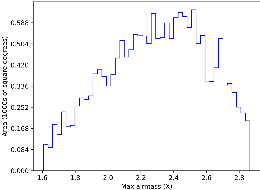
too_elab_r64_d2_giz_v3.4_10yrs WFD y band: Max airmass
