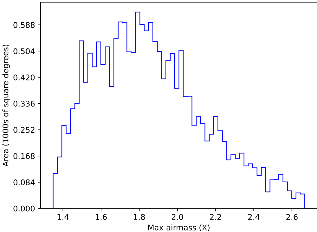
too_elab_r64_d2_giz_v3.4_10yrs WFD u band: Max airmass
