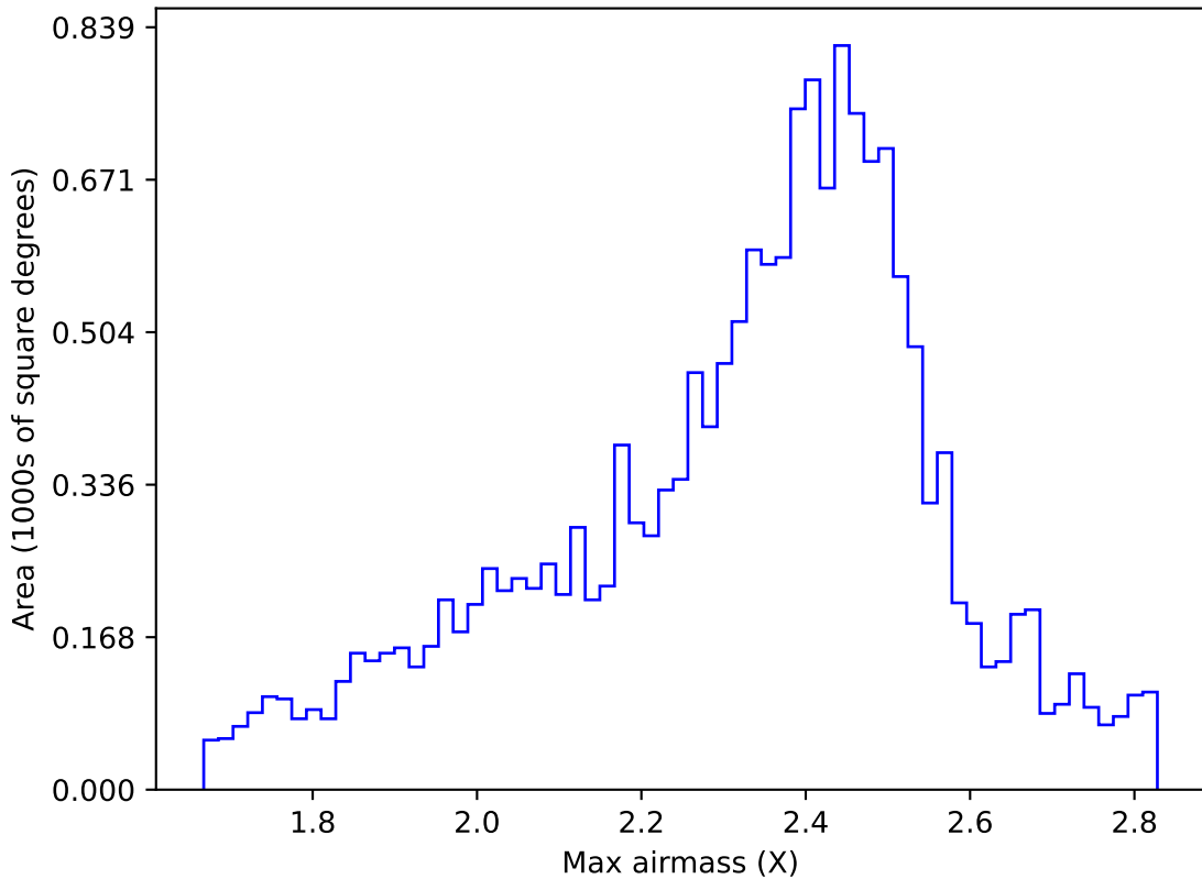
too_elab_r64_d2_giz_v3.4_10yrs WFD r band: Max airmass
