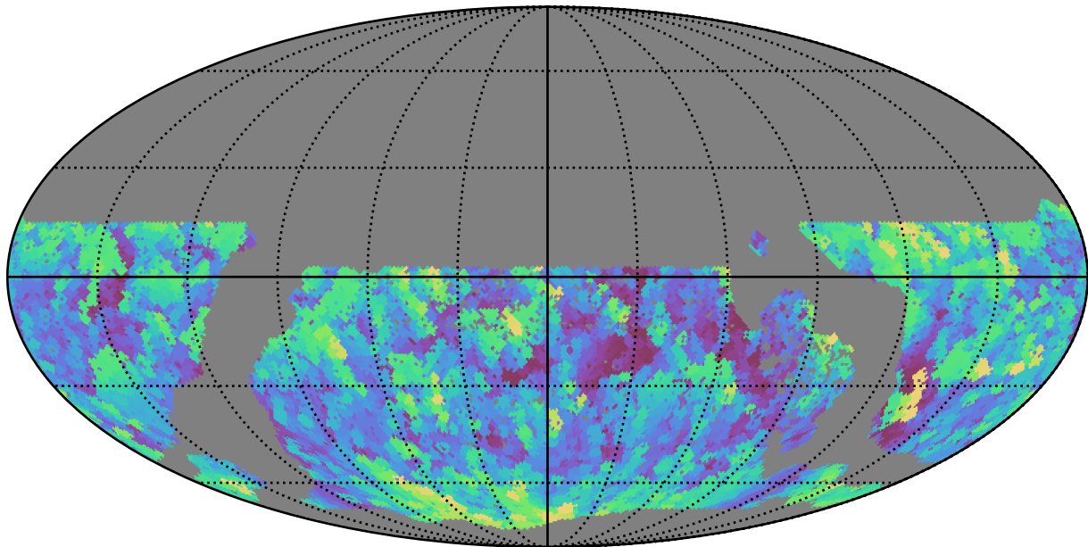
too_elab_r64_d2_giz_v3.4_10yrs WFD g band: Max airmass
