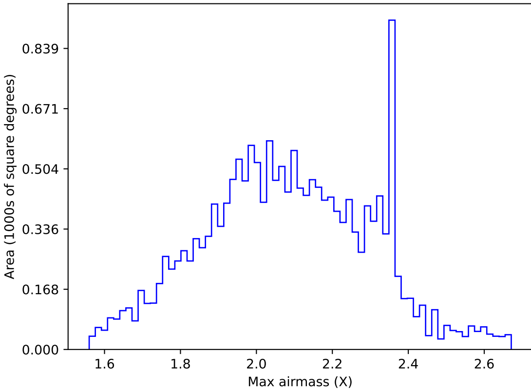
too_elab_r64_d2_giz_v3.4_10yrs WFD g band: Max airmass
