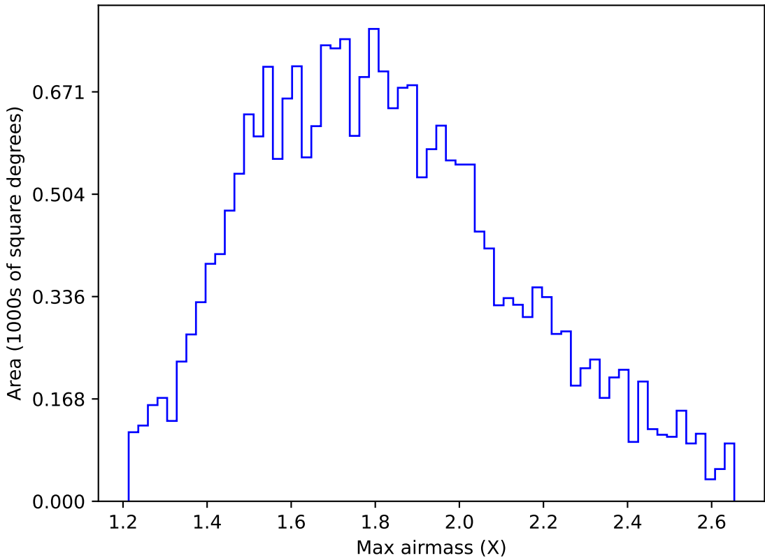
too_elab_r64_d2_giz_v3.4_10yrs All sky u band: Max airmass
