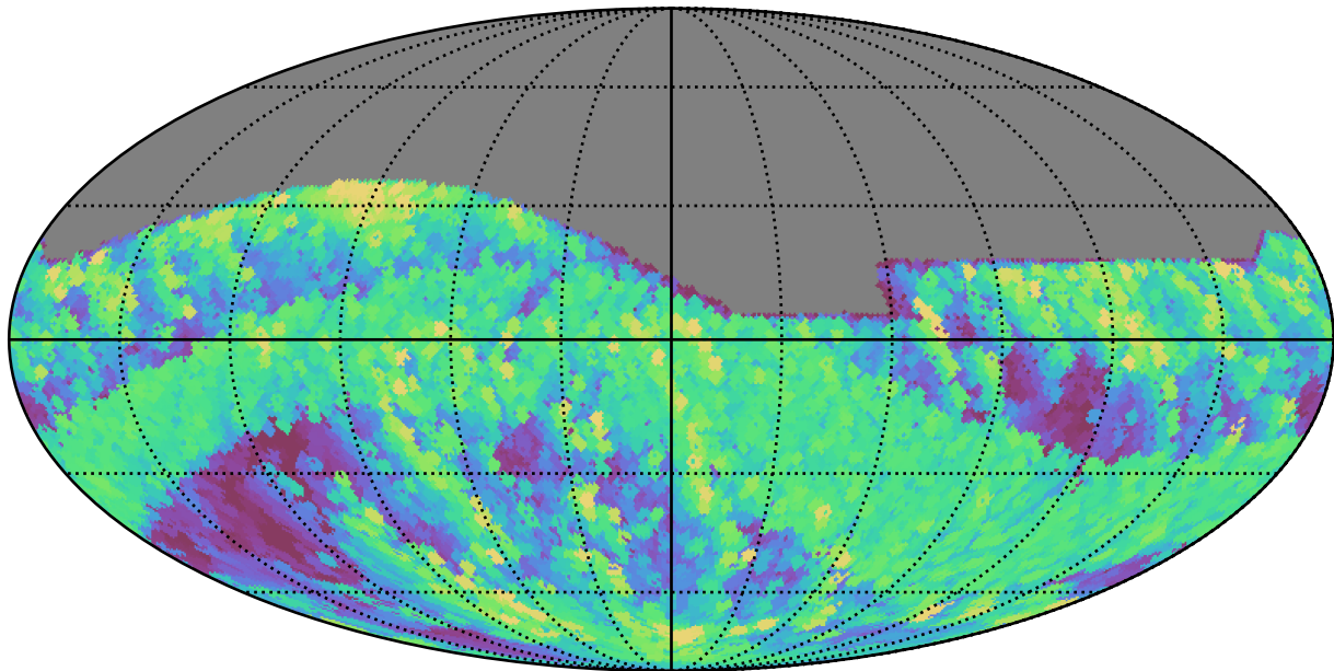
too_elab_r64_d2_giz_v3.4_10yrs All sky r band: Max airmass
