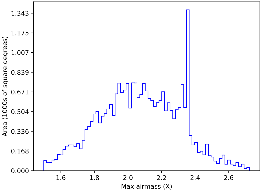
too_elab_r64_d2_giz_v3.4_10yrs All sky g band: Max airmass
