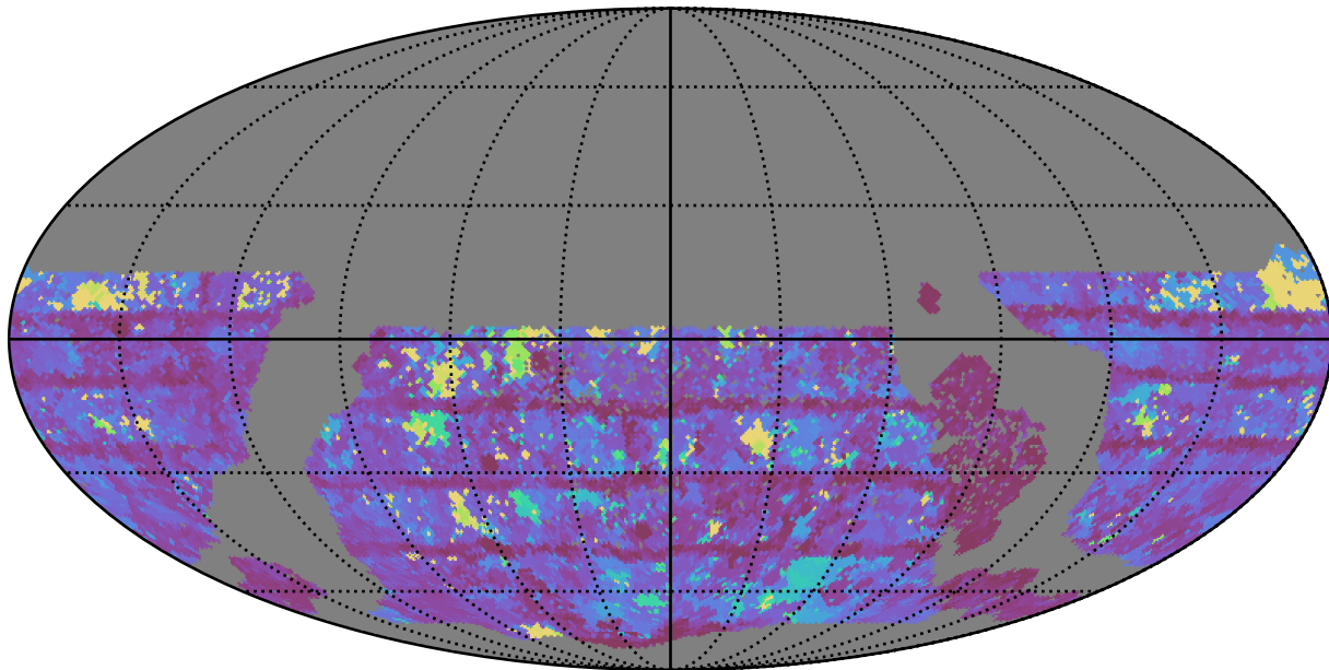
too_elab_r64_d2_giz_v3.4_10yrs WFD z band: Max Inter-Night Gap
