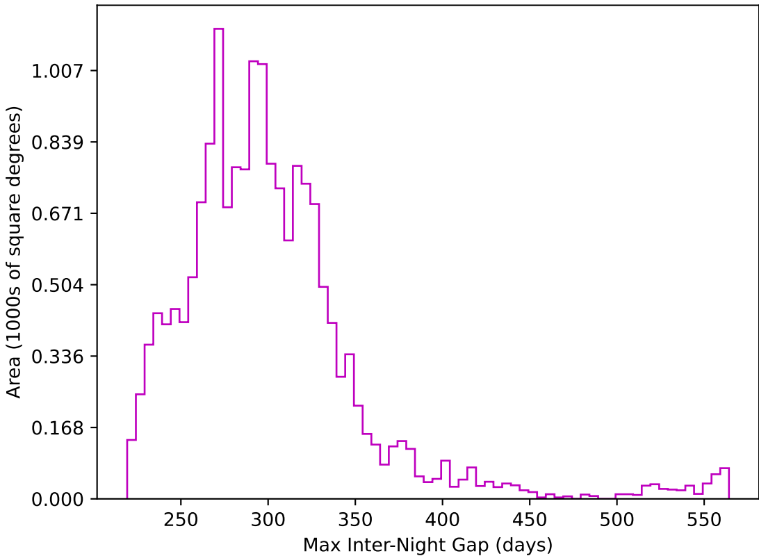
too_elab_r64_d2_giz_v3.4_10yrs WFD z band: Max Inter-Night Gap
