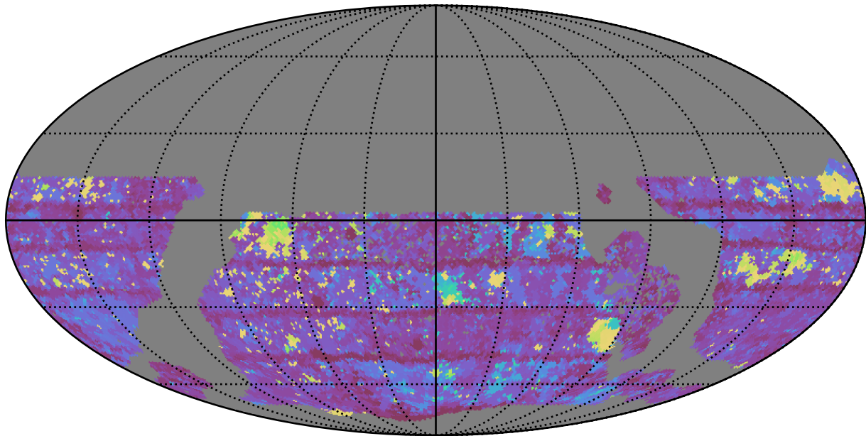
too_elab_r64_d2_giz_v3.4_10yrs WFD y band: Max Inter-Night Gap
