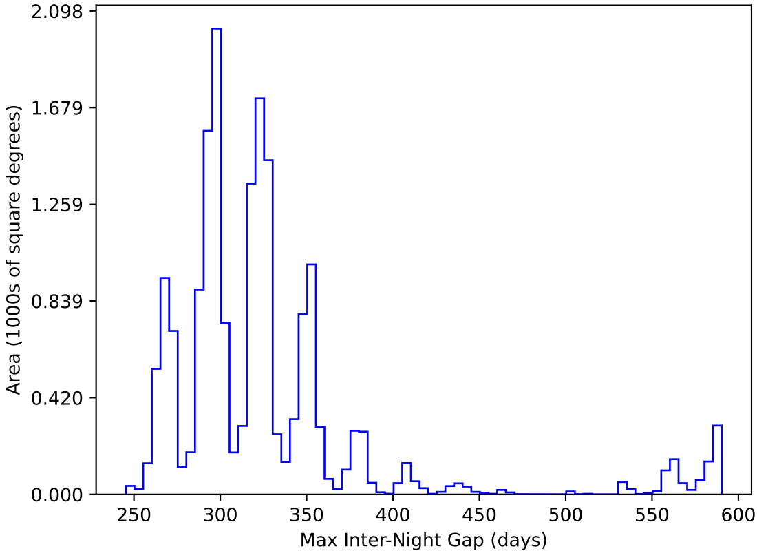
too_elab_r64_d2_giz_v3.4_10yrs WFD y band: Max Inter-Night Gap
