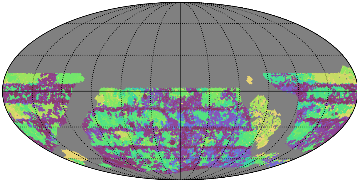
too_elab_r64_d2_giz_v3.4_10yrs WFD u band: Max Inter-Night Gap
